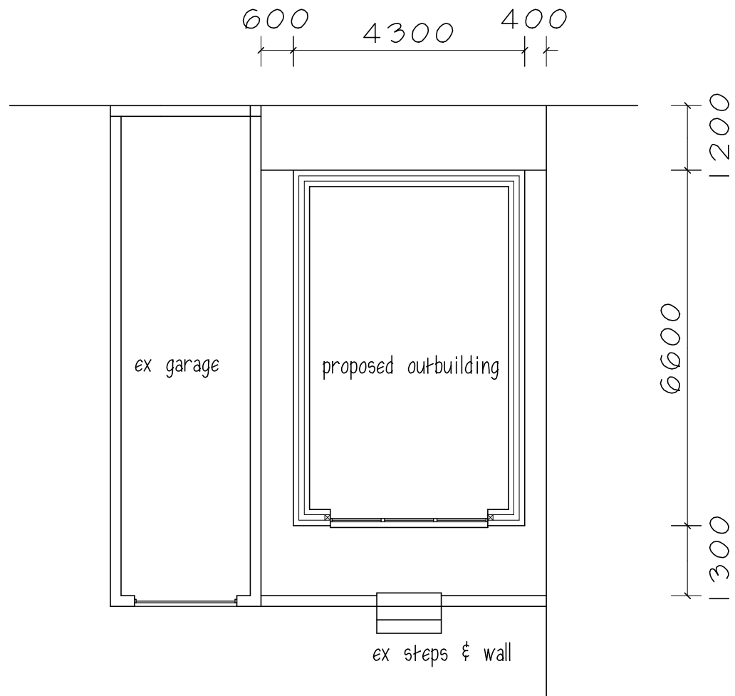
PLAN
