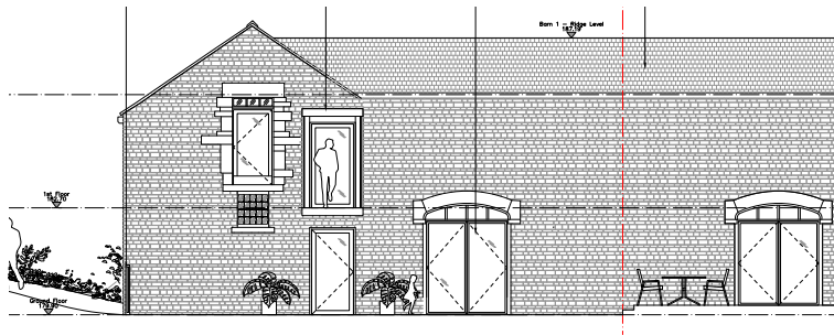
ORIGINAL APPLICATION SUBMISSION - ARCH BARN- GARDEN ELEVATION
