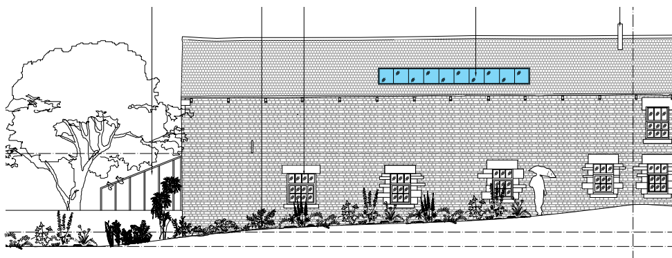
ORIGINAL APPLICATION SUBMISSION - BARN 1 - EASTFIELD LN ELEVATION
