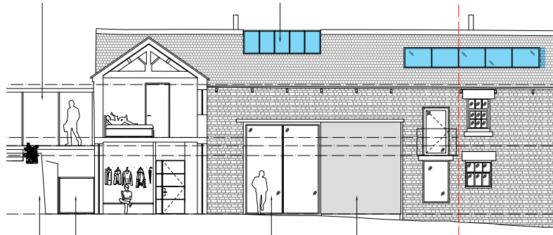
ORIGINAL APPLICATION SUBMISSION - BARN 1 - COURTYARD ELEVATION
