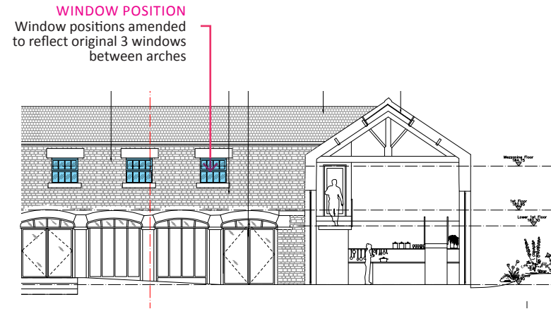
AMENDED APPLICATION SUBMISSION - ARCH BARN- COURTYARD ELEVATION
