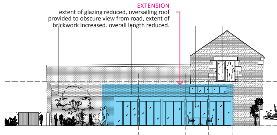
ORIGINAL APPLICATION SUBMISSION - BARN 1 - EASTFIELD LN ELEVATION
