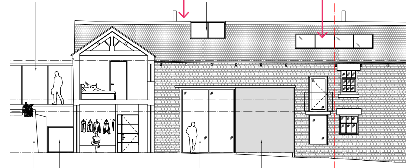
AMENDED APPLICATION SUBMISSION - BARN 1 - COURTYARD ELEVATION
