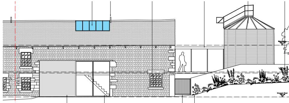
ORIGINAL APPLICATION SUBMISSION - BARN 1 - EASTFIELD LN ELEVATION
