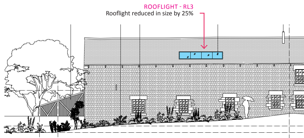
ORIGINAL APPLICATION SUBMISSION - BARN 1 - EASTFIELD LN ELEVATION
