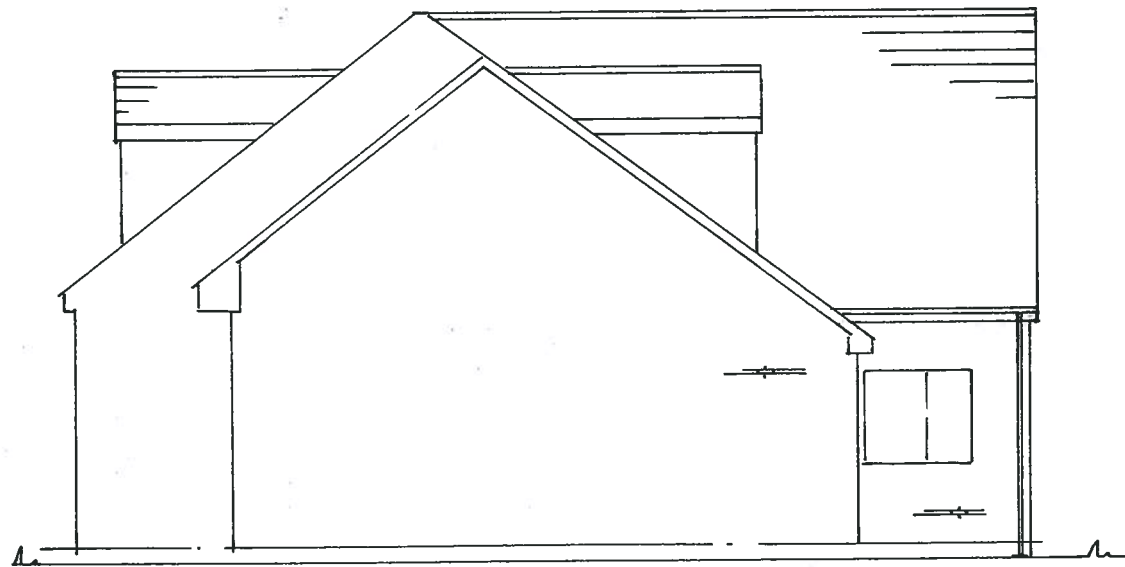
PROPOSED ELEVATION ON '3'
