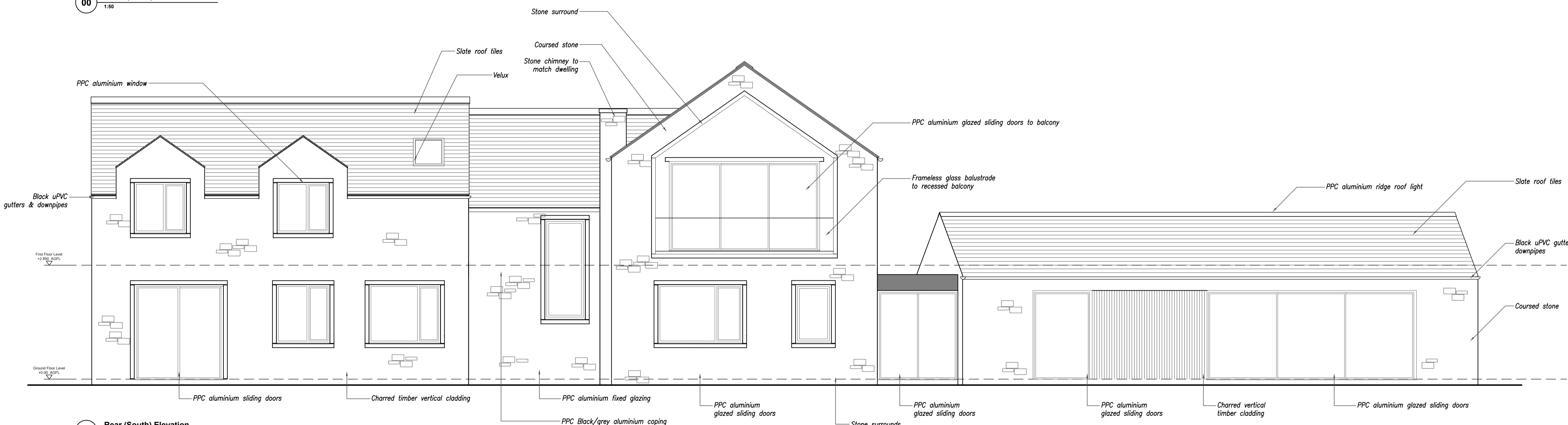
00 Rear (South) Elevation 1:50
