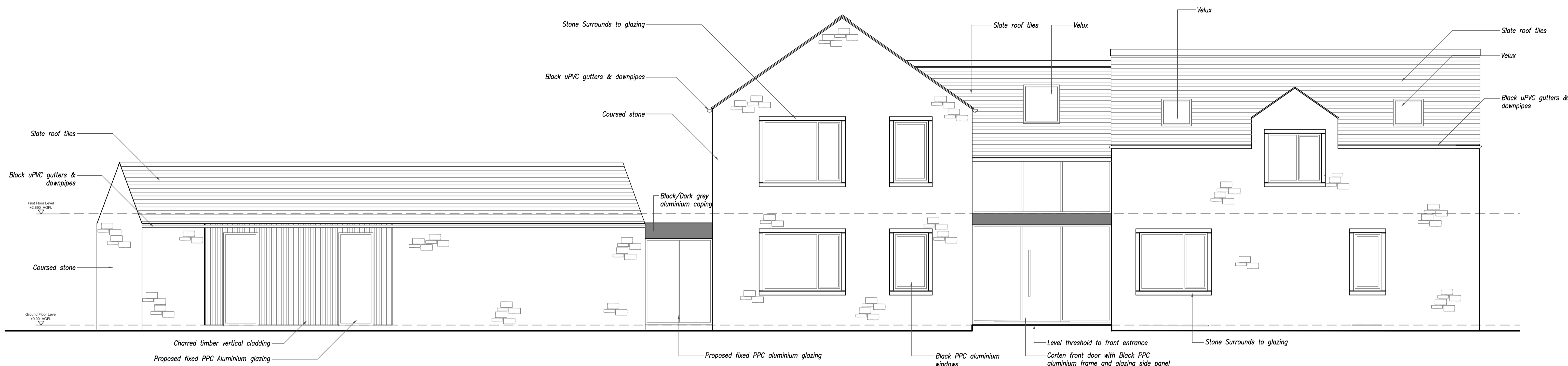
00 Front (North) Elevation 1:50
