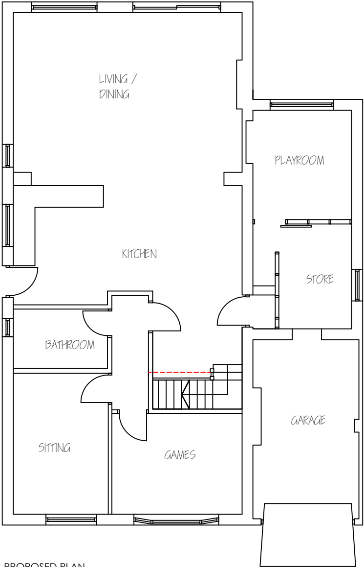
PROPOSED PLAN 1:100
