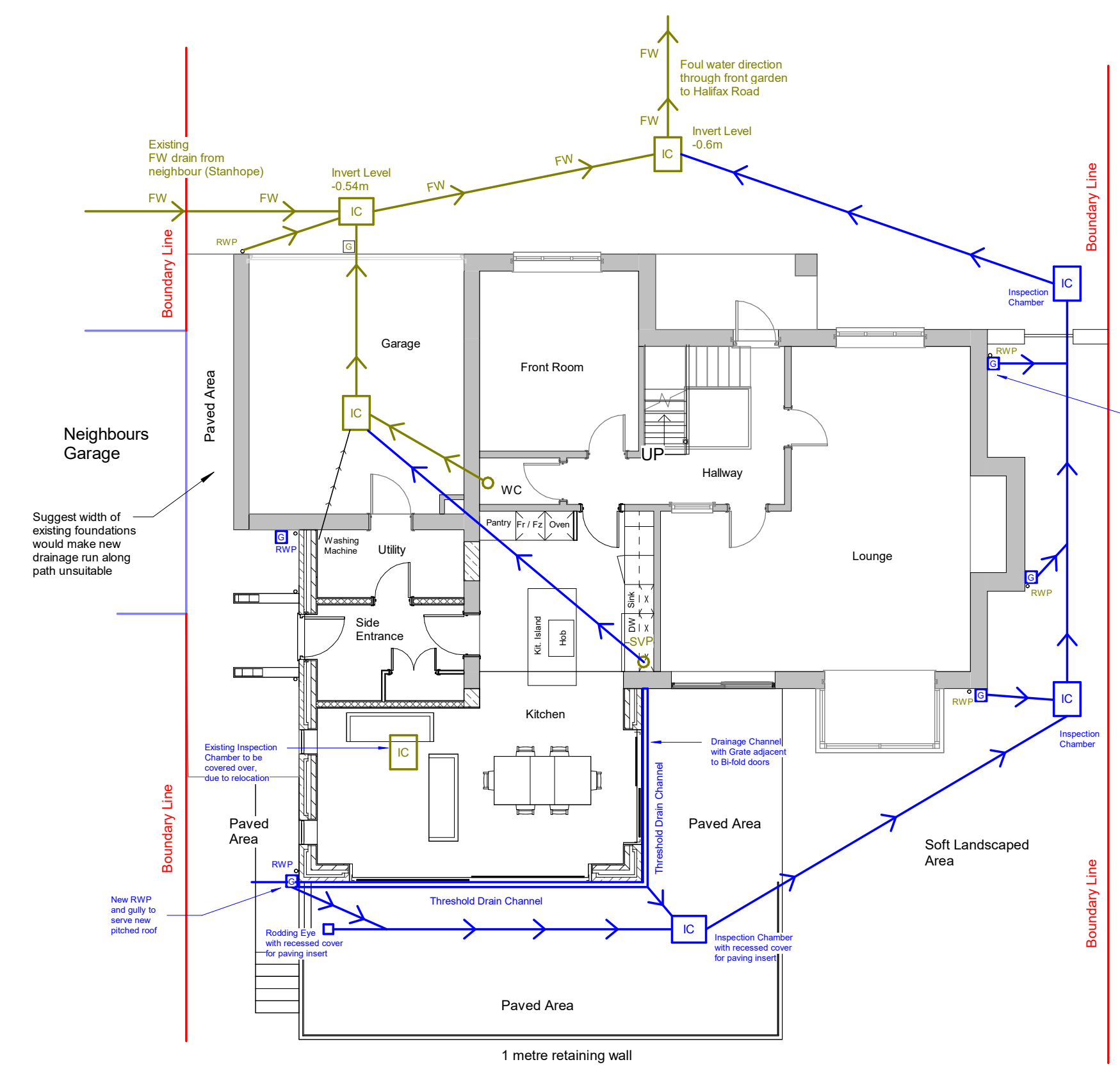
3 Proposed Drainage Plan 1 : 100
