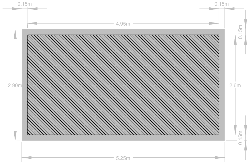
Floorplan showing base and garage exterior dimensions
