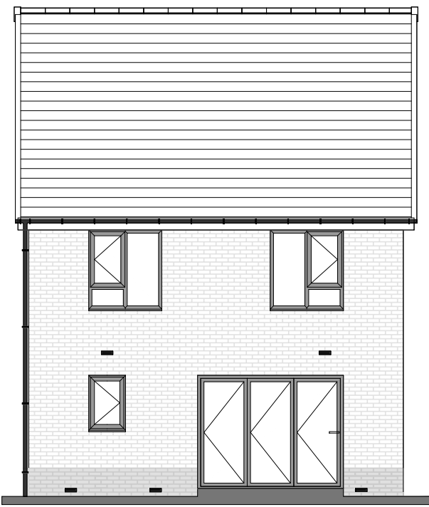
REAR ELEVATION
