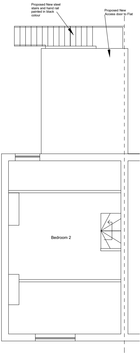
EXISTING SECOND FLOOR PLAN
