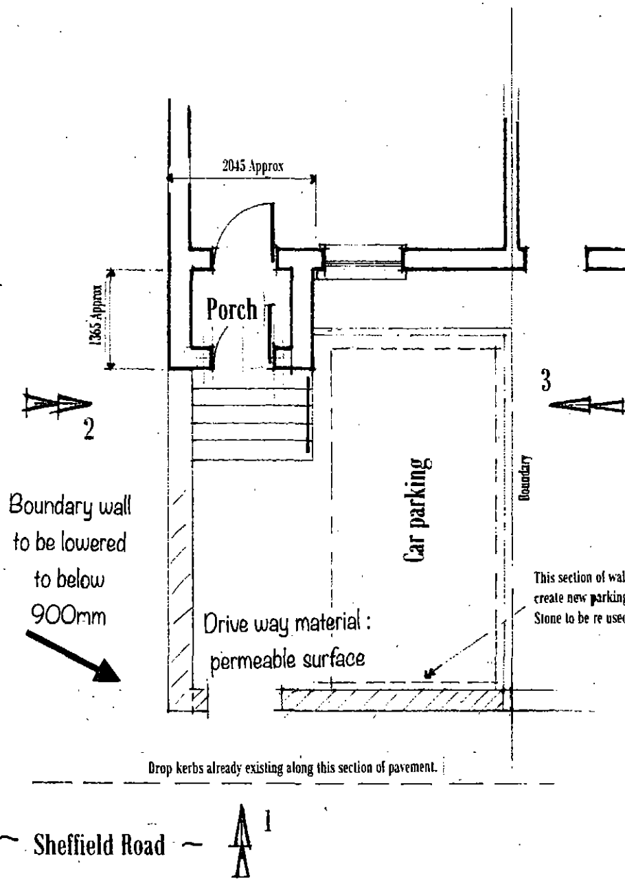
Proposed details of Front driveway + porch Scale 1 : 50
