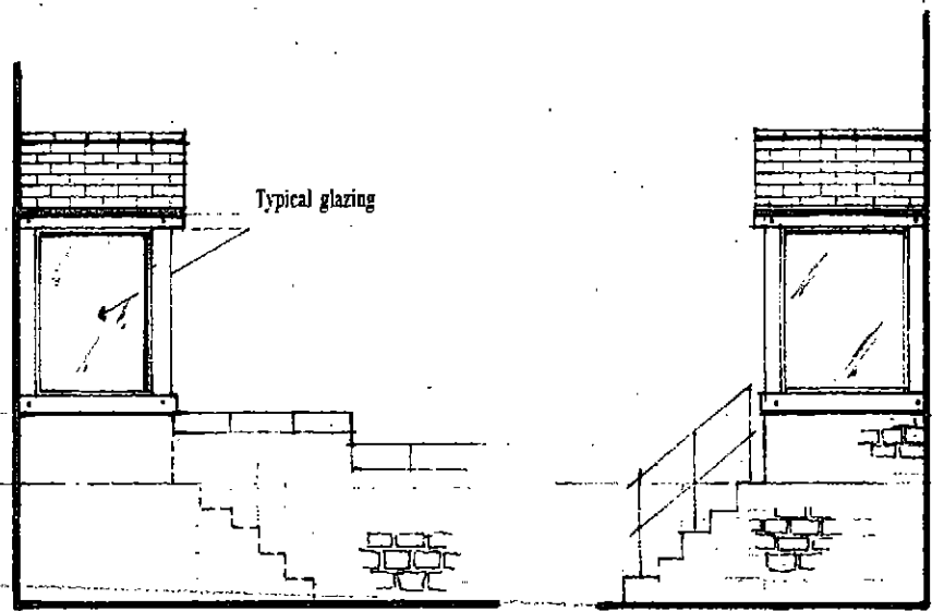
Proposed Elevation On Arrow 2
