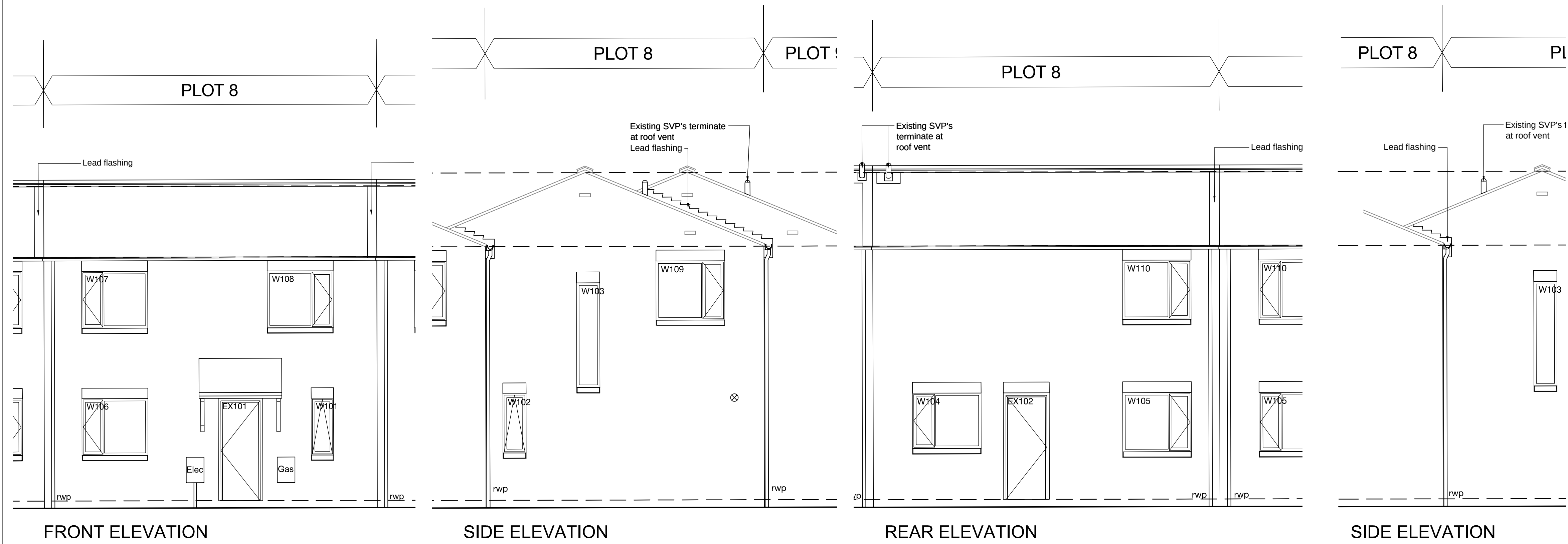
PLOT 08 EXISTING ELEVATIONS
