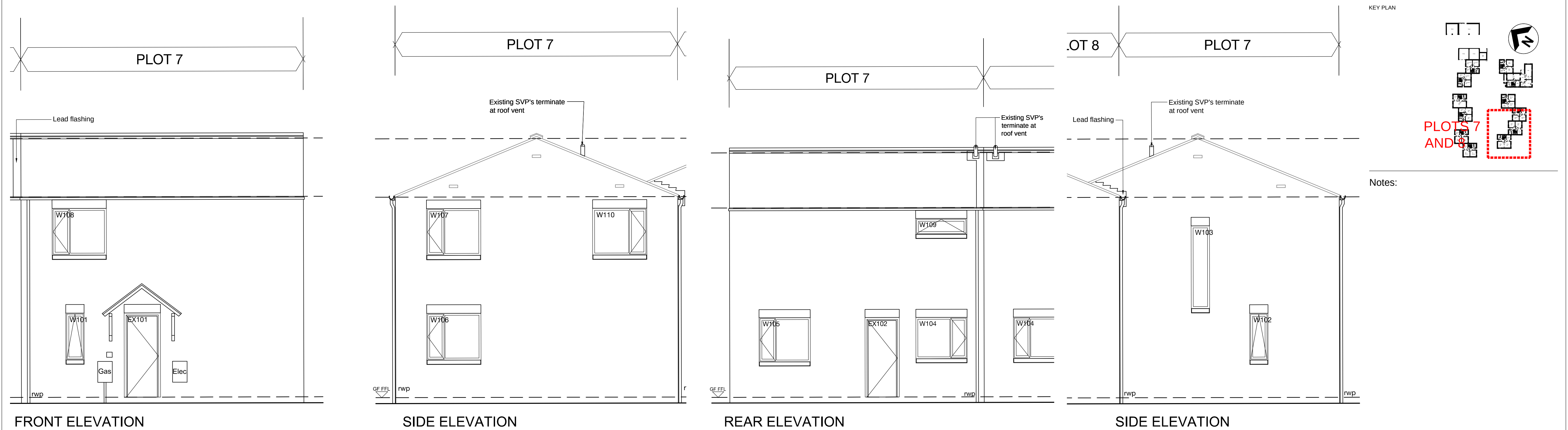
PLOT 07 EXISTING ELEVATIONS
