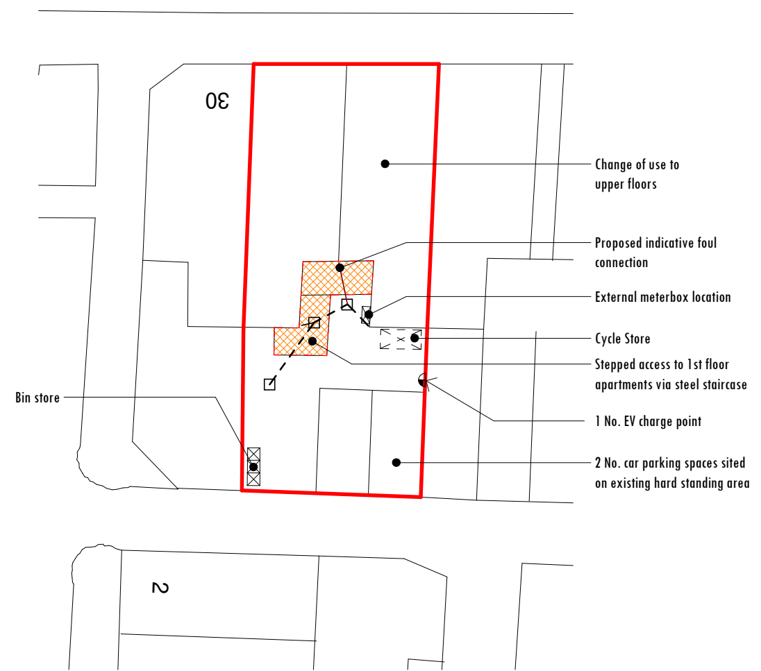
3 Proposed Site Plan 1 : 250
