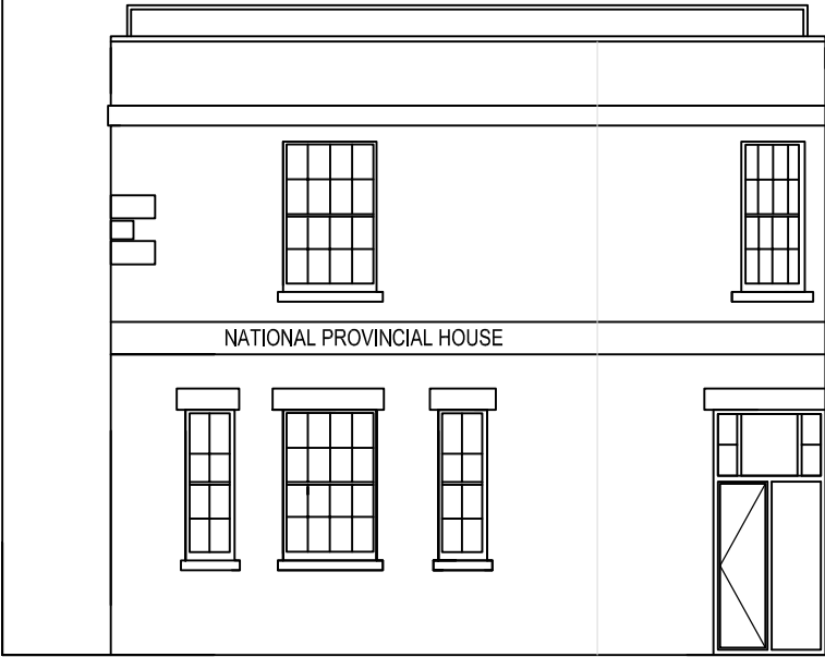
PROPOSED SOUTH ELEVATION
