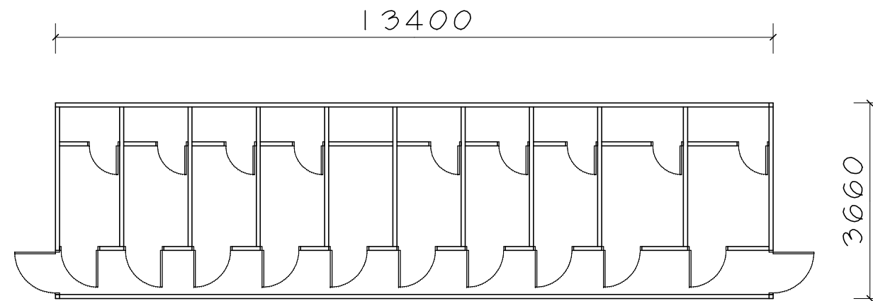
FLOOR PLAN
