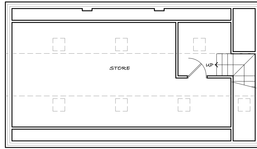
PROPOSED FIRST FLOOR PLAN 1/100
