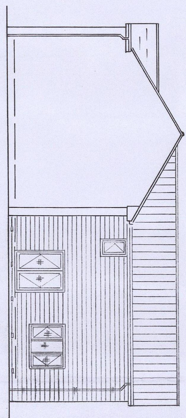
PROPOSED SIDE NORTH
