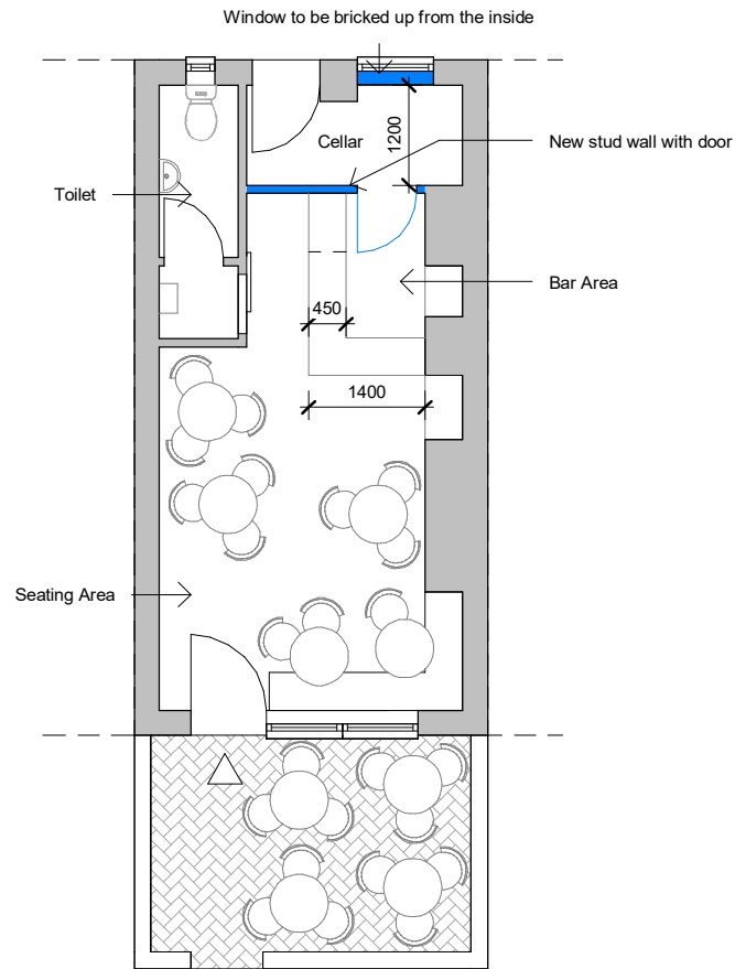
Proposed Plan
