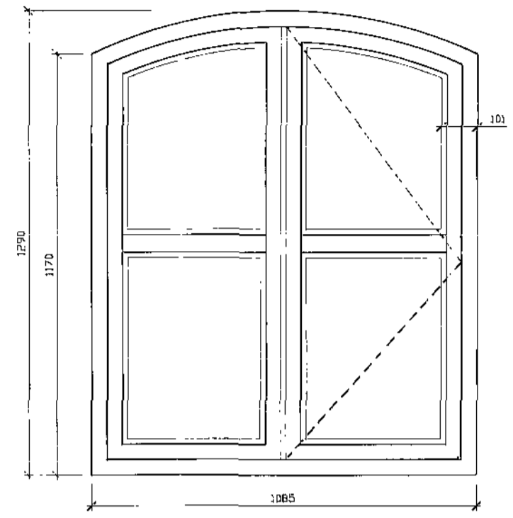
End Bedroom Window (opening window on right)
