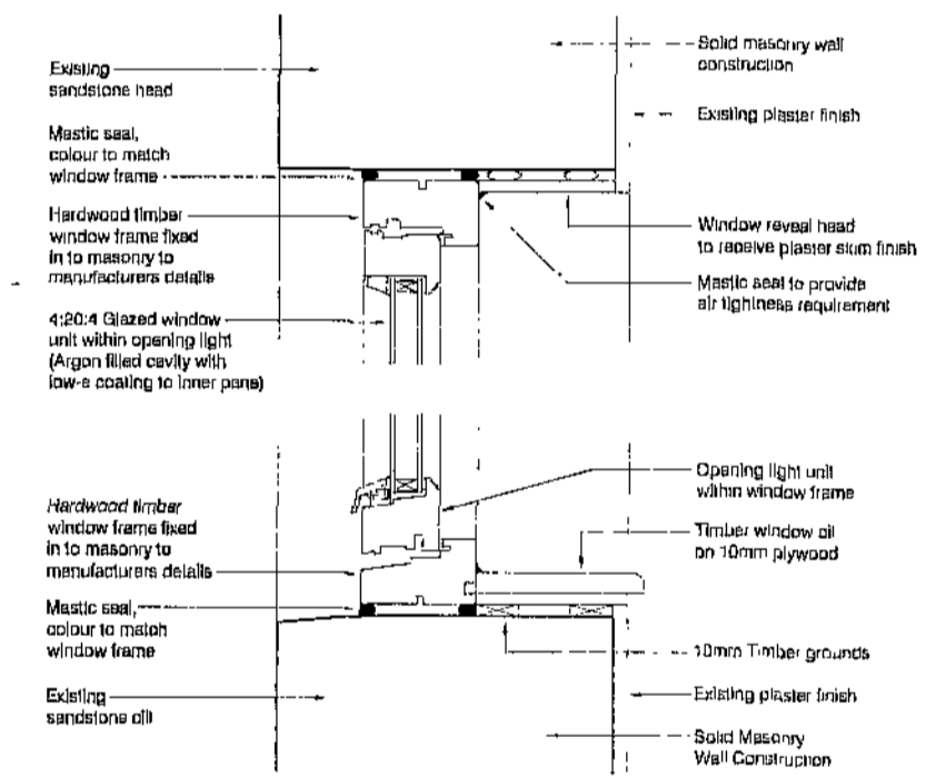
Opening Window Frame Section Scale - 1:5
