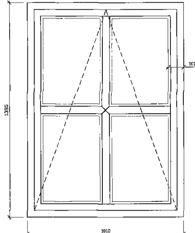
Lounge Window - facing garden (top hinged opening window)
