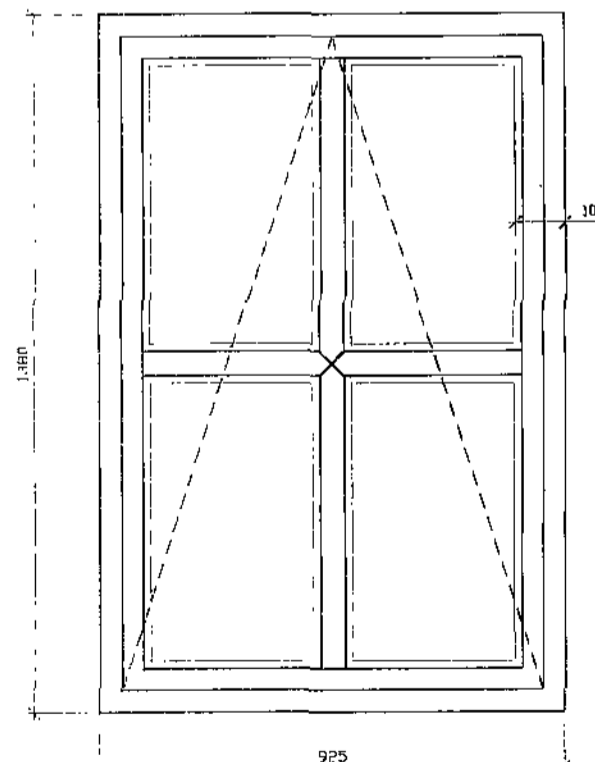
Lounge Window - facing road (top hinged opening window)
