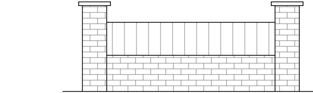
EXISTING FRONT ELEVATION
