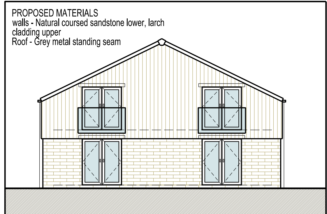
East Elevation
