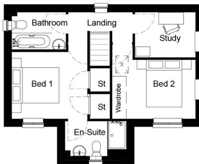
First Floor. 1 : 100
