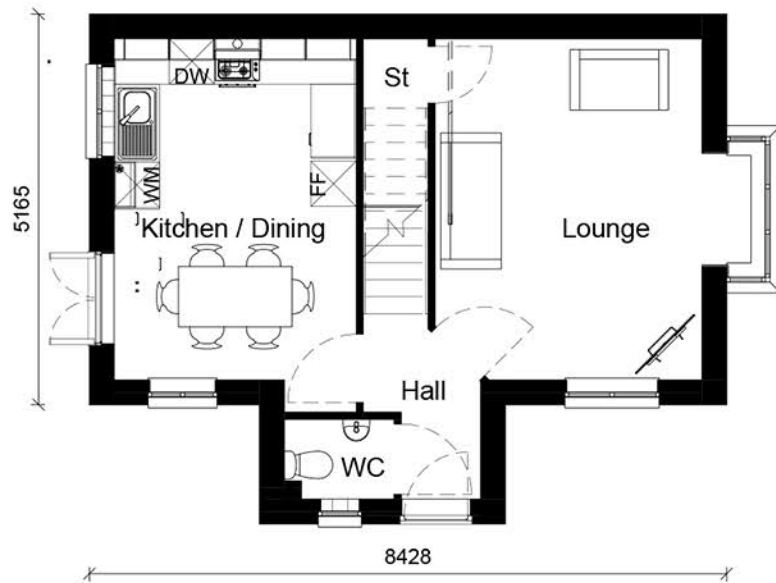
Ground Floor. 1 : 100
