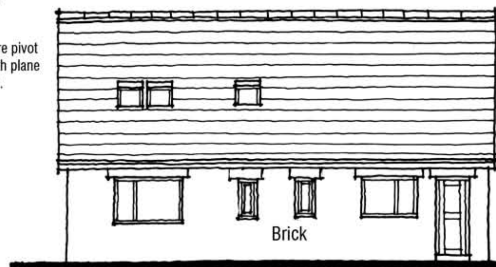
West Elevation
