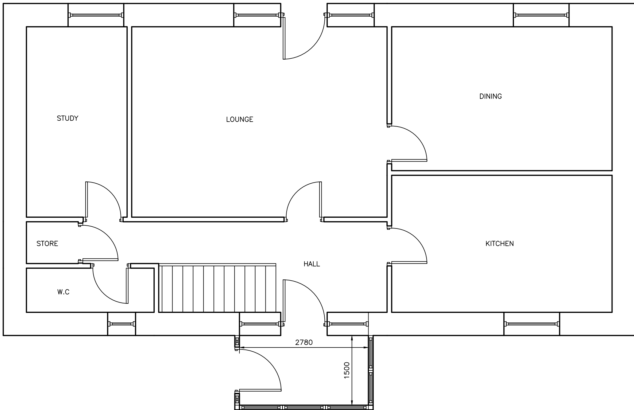
PROPOSED PLAN
