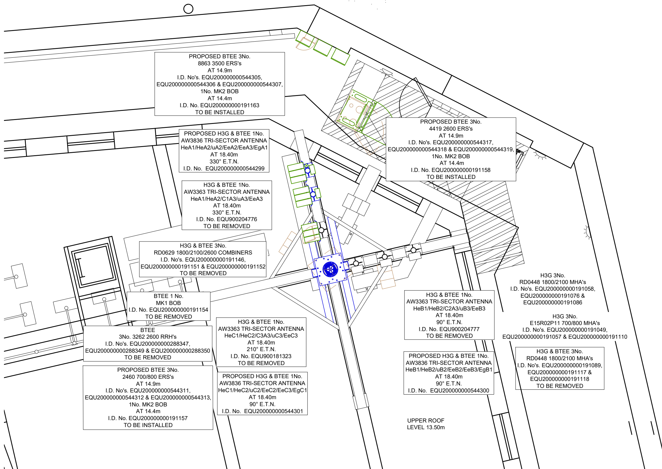
ANTENNA PLAN AT 18.40m
