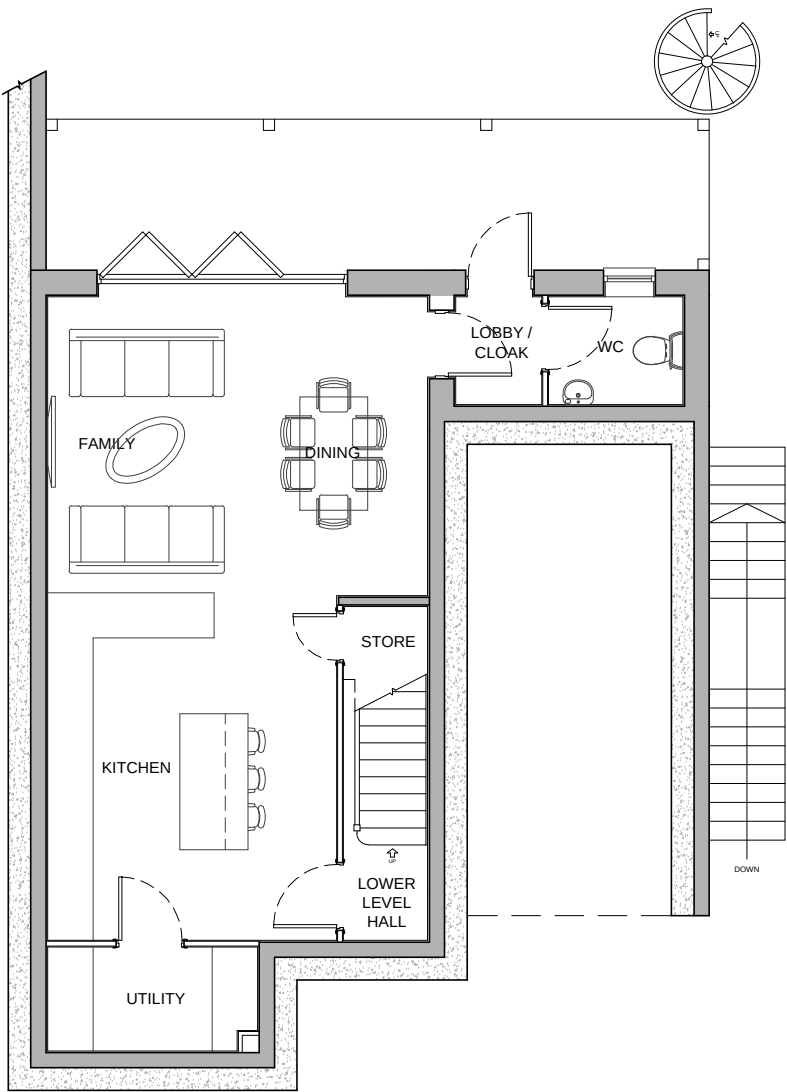
LOWER GROUND FLOOR PLAN
