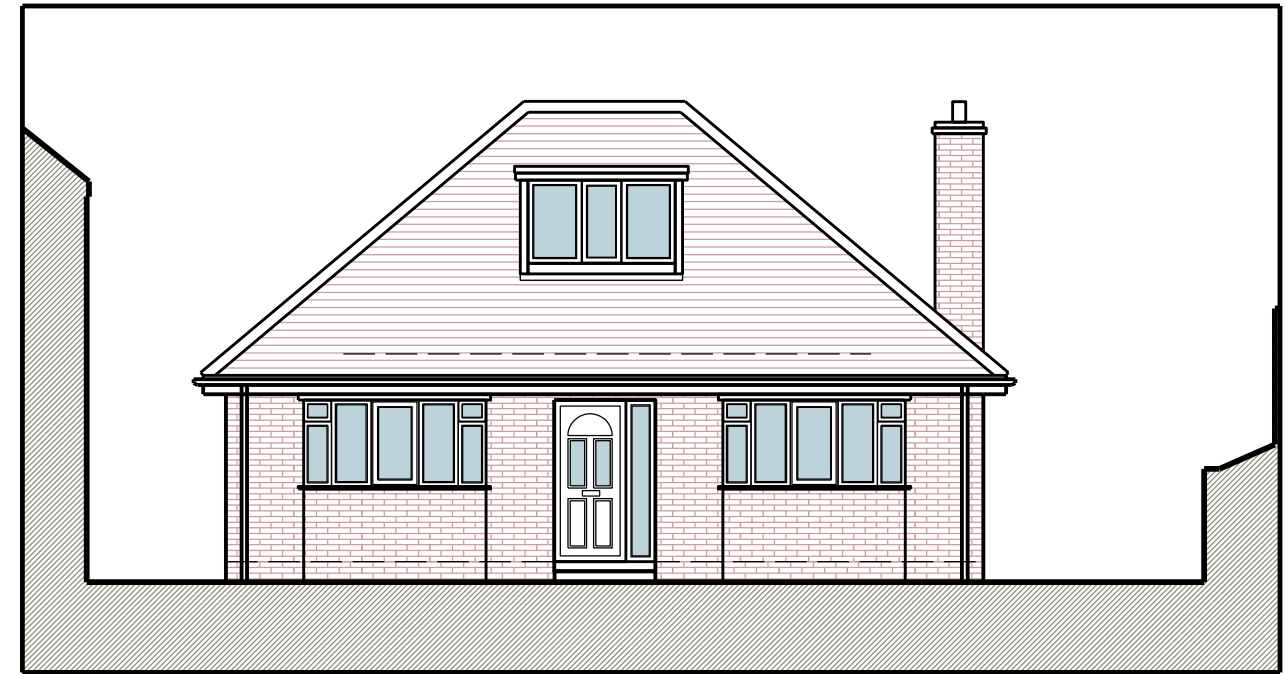
East Elevation
