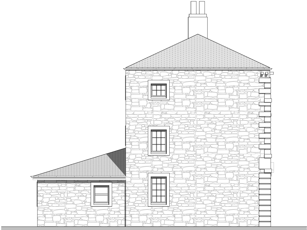
E-04 Existing Side Elevation 1:100
