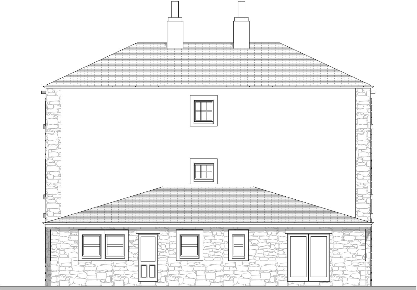
E-03 Existing Rear Elevation
