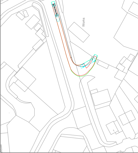
Articulated Vehicle left turn 1:500
