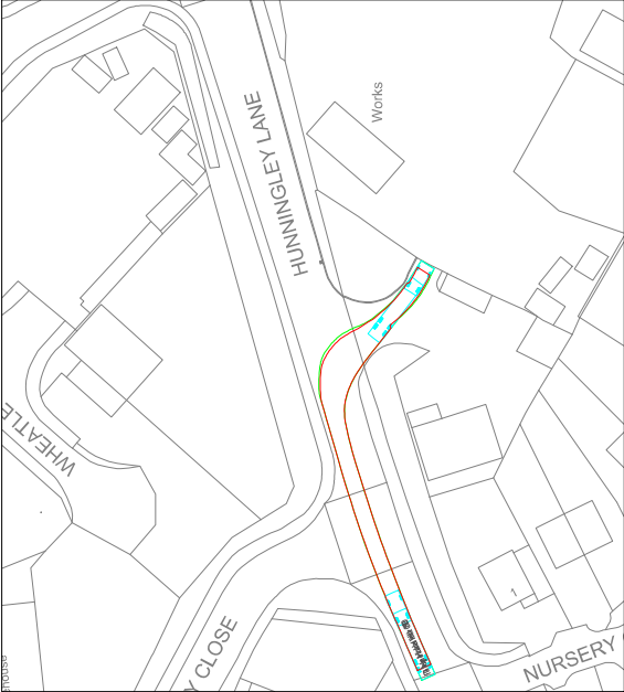
Articulated Vehicle right turn 1:500
