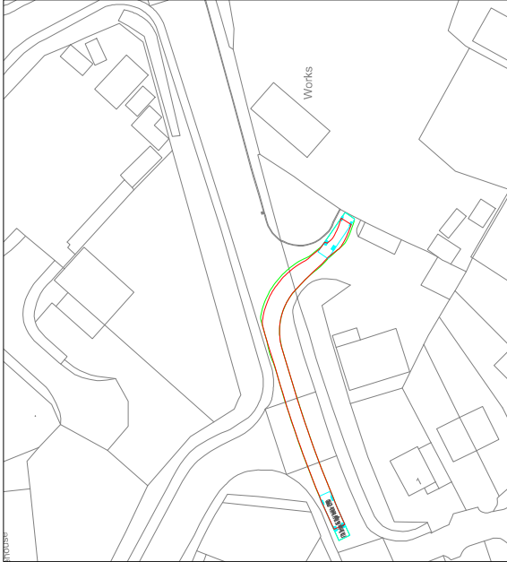
HG Rigid Vehicle right turn 1:500
