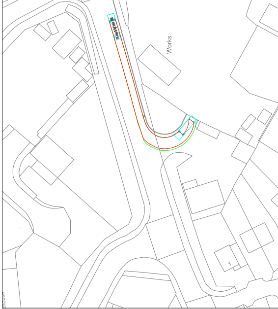
HG Rigid Vehicle left turn 1:500
