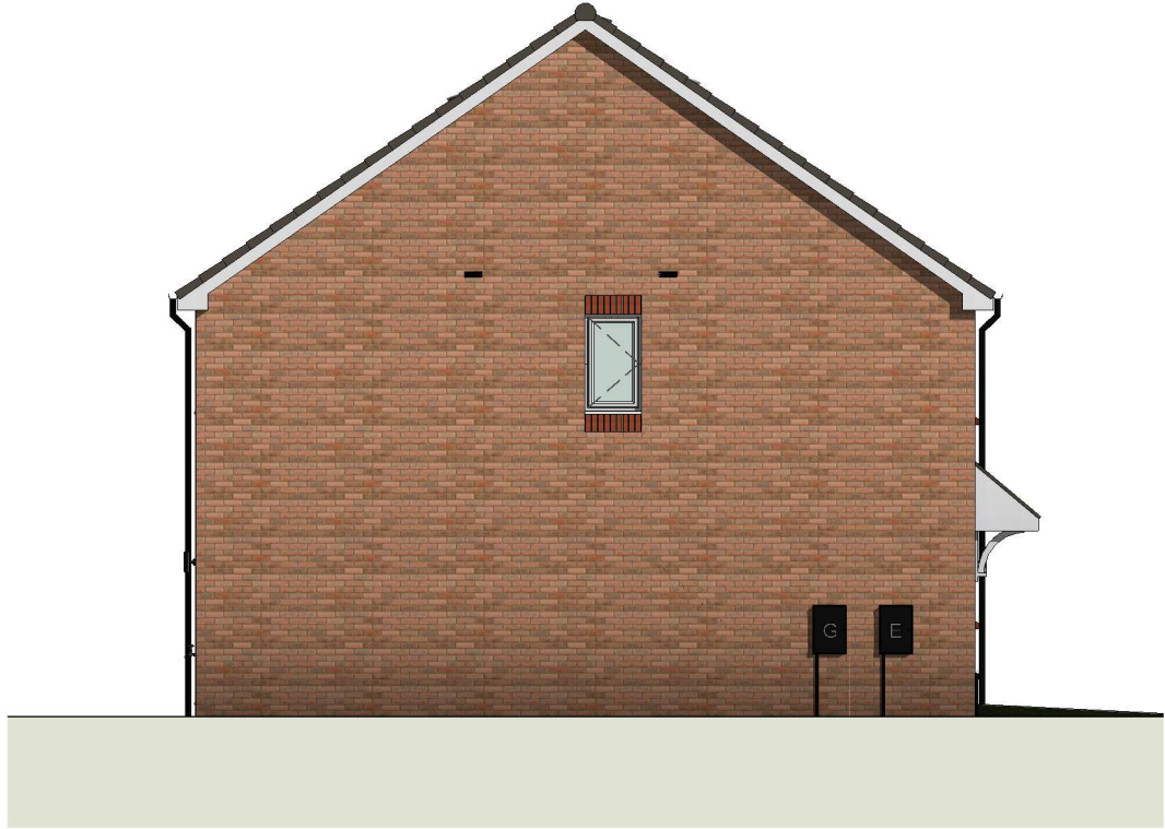
2 Gable Elevation 1 : 100
