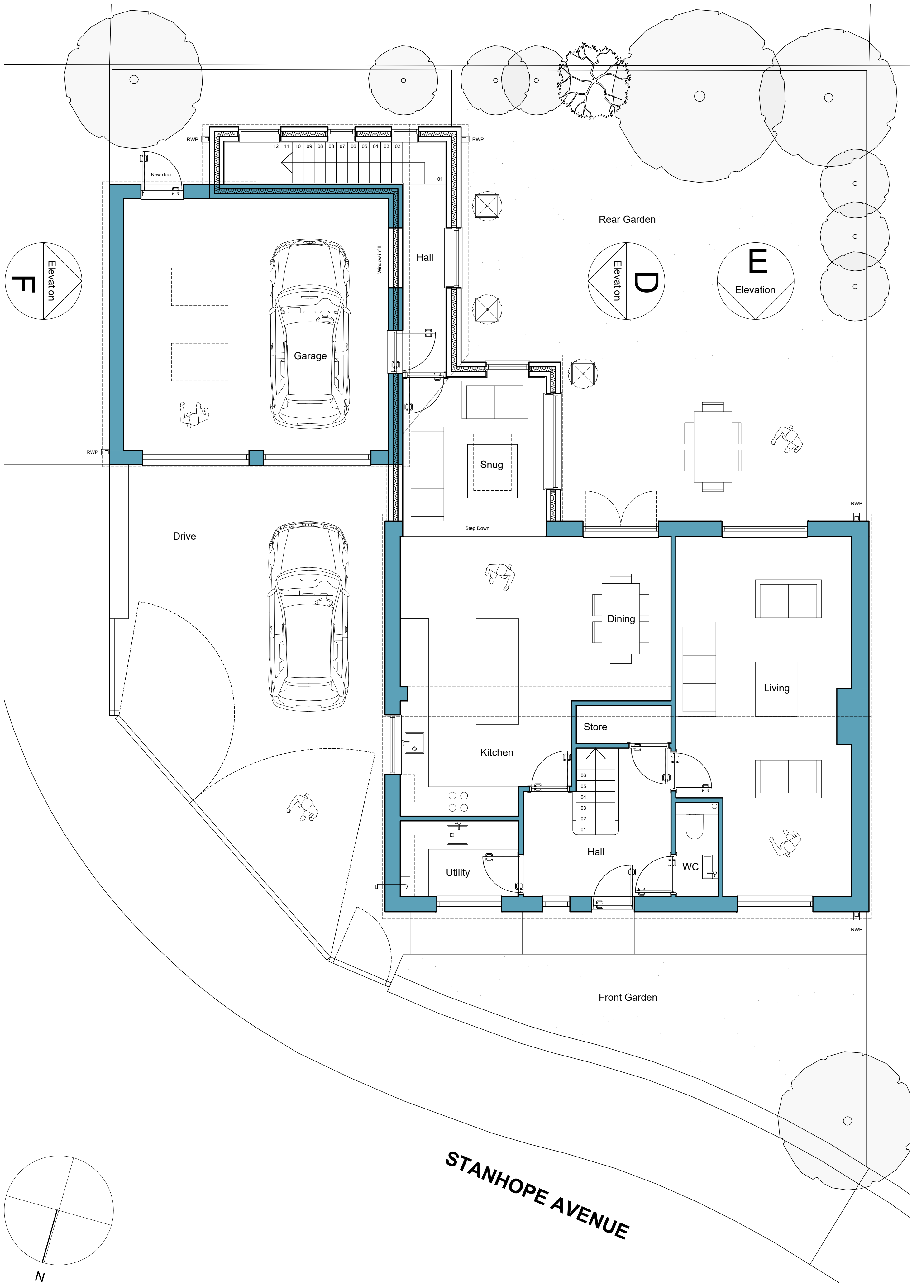
Proposed Ground Floor Plan 1:50 @ A1
