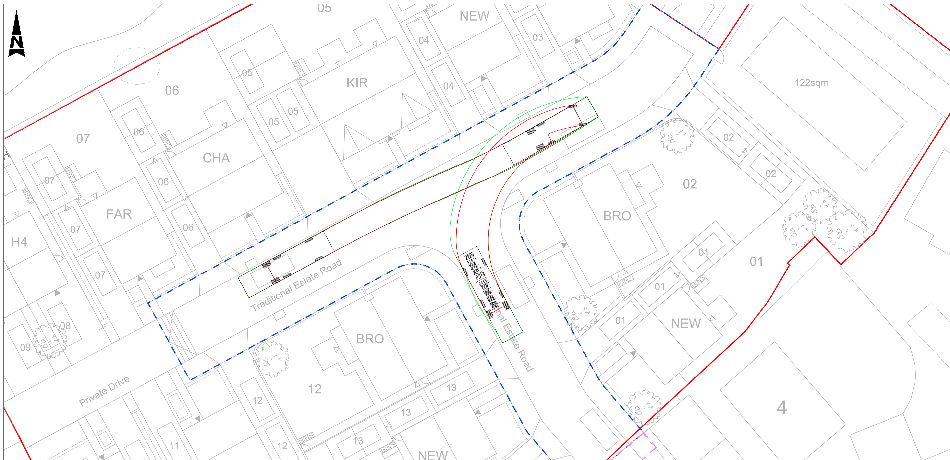
REFUSE VEHICLE TRACKING 1 SCALE 1:200
