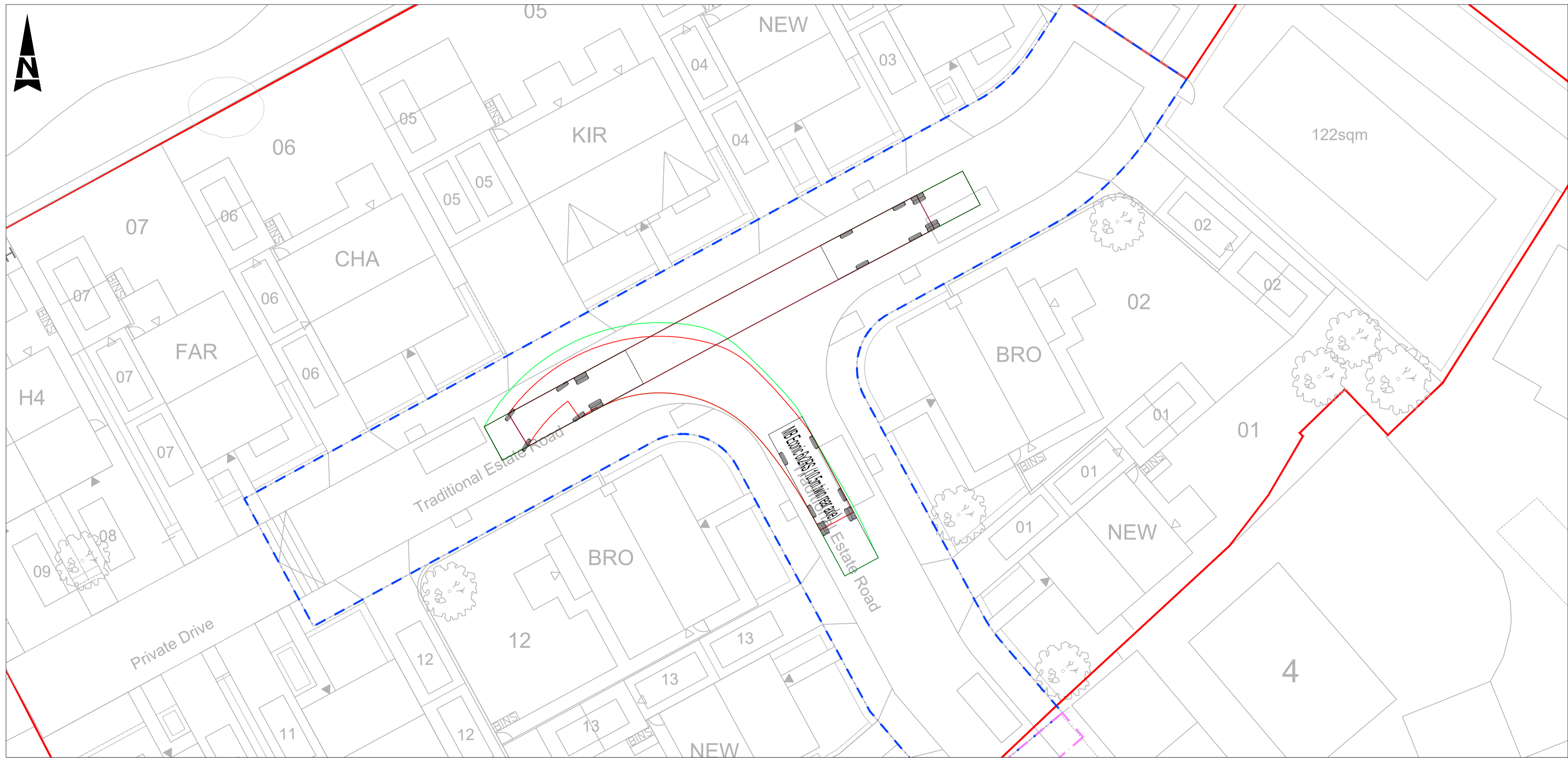
REFUSE VEHICLE TRACKING 2 SCALE 1:200
