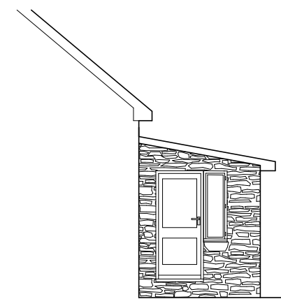
SIDE ELEVATION
