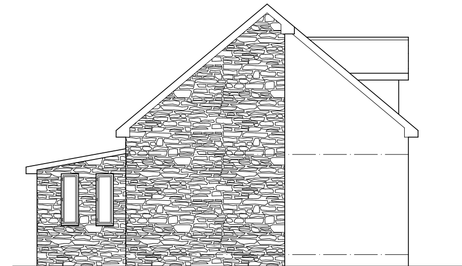
SIDE ELEVATION
