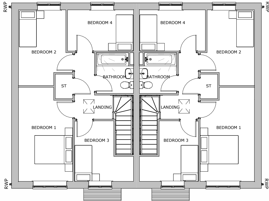
First Floor 1 : 100
