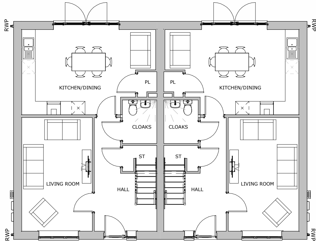
Ground Floor 1 : 100
