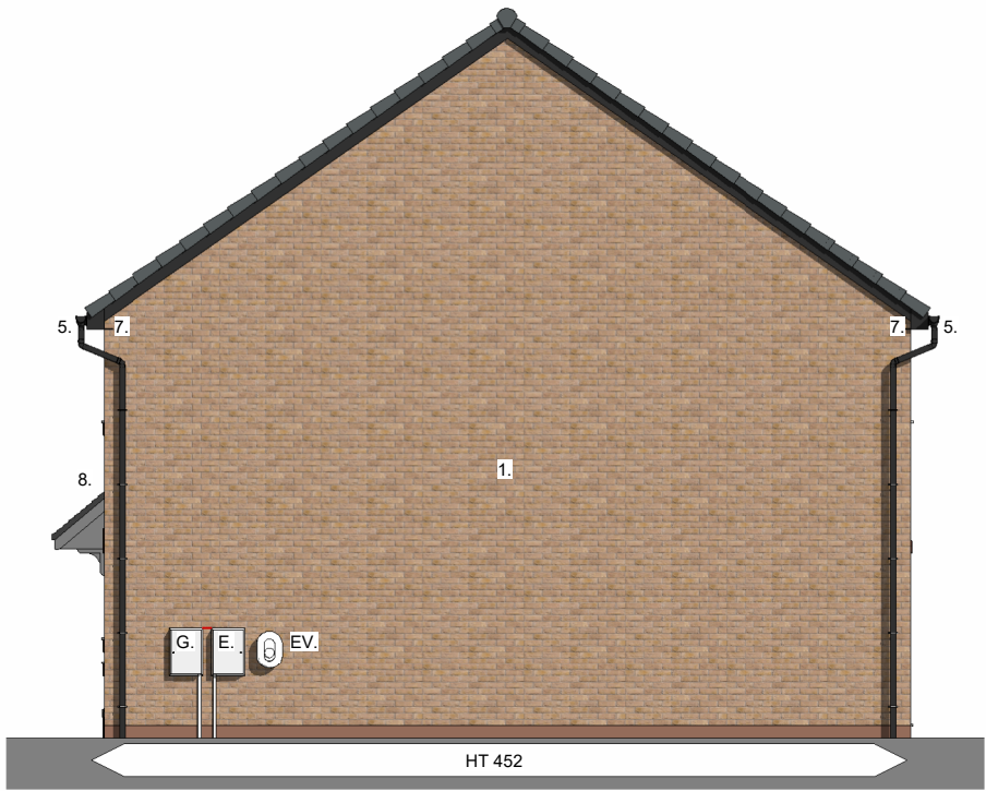
Side Elevation 1 : 100
