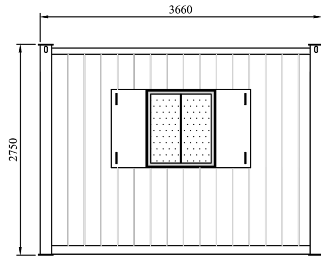
GABLE ELEVATION
