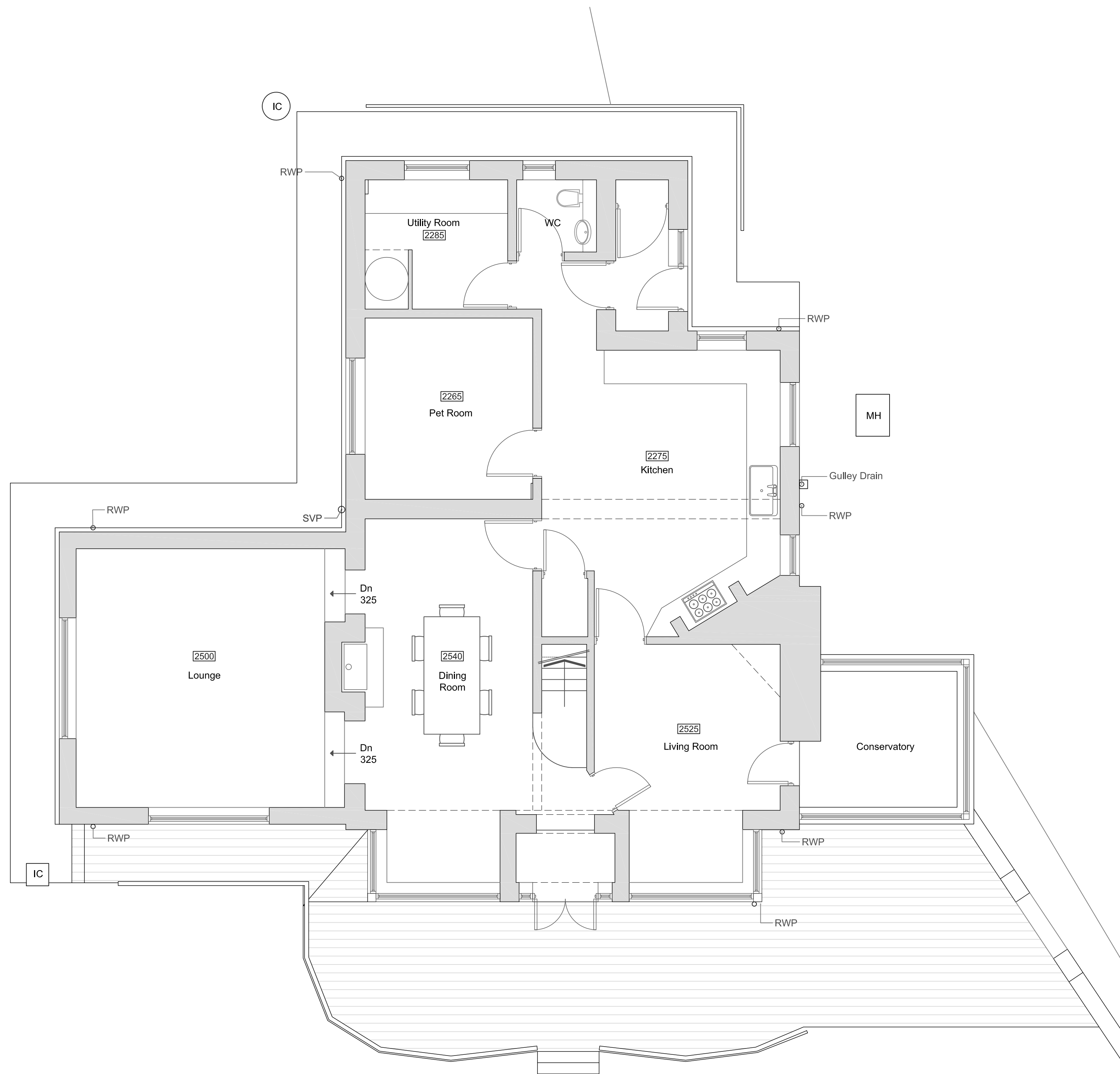
Ground Floor GA Scale 1: 50
