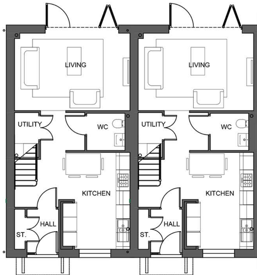
GROUND FLOOR PLAN Lorton (end)
