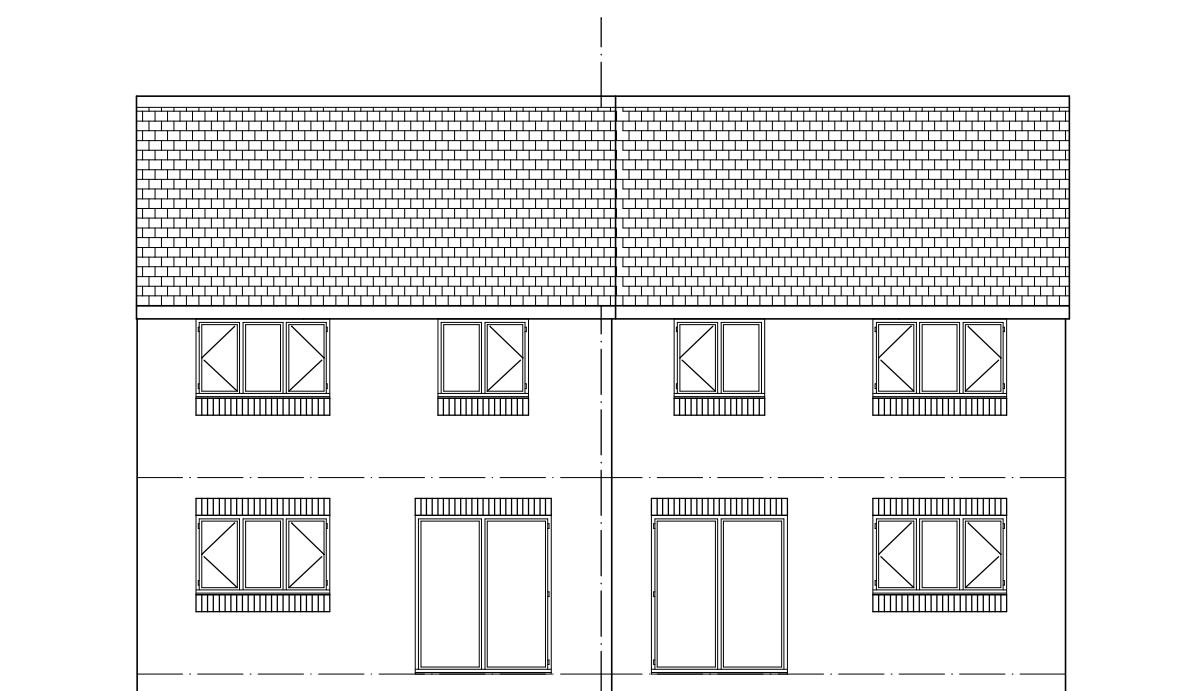
REAR ELEVATION
