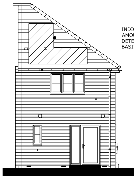
REAR
