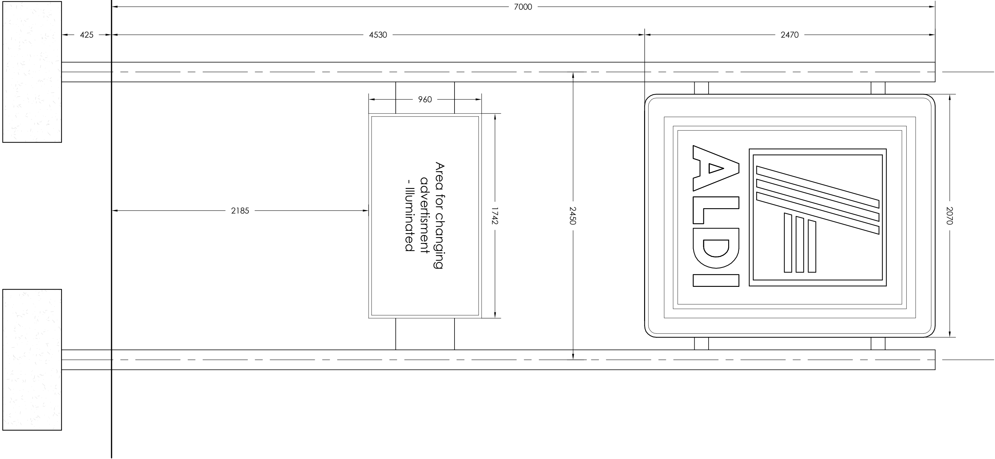
PROPOSED ILLUMINATED FREESTANDING SIGN SIGN 1
