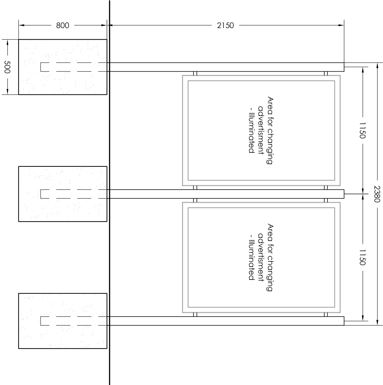
PROPOSED ILLUMINATED FREESTANDING POSTER SIGN SIGN 4
