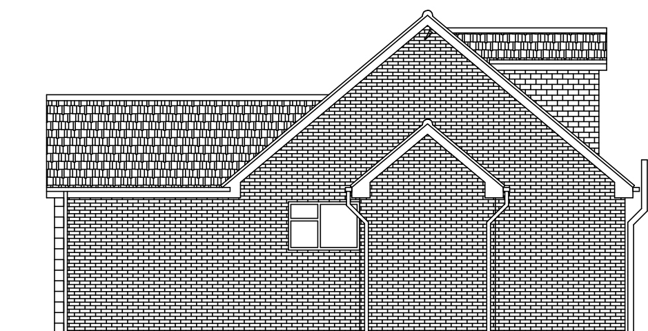
END ELEVATION SCALE 1:100
