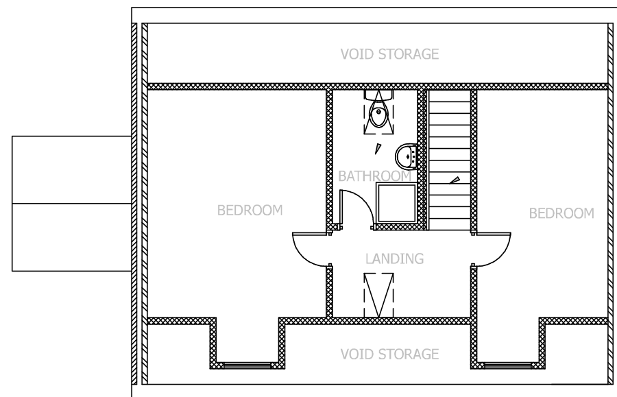
FIRST FLOOR PLAN SCALE 1:100 AT A3
