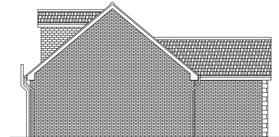
END ELEVATION SCALE 1:100
