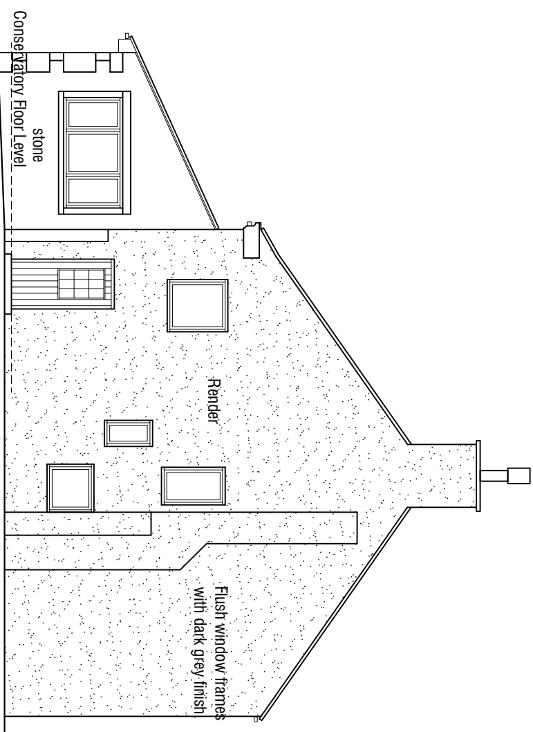
South Elevation 1:100
