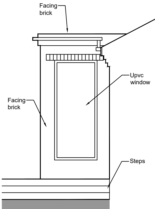
EXISTING SIDE ELEVATION 1:50
