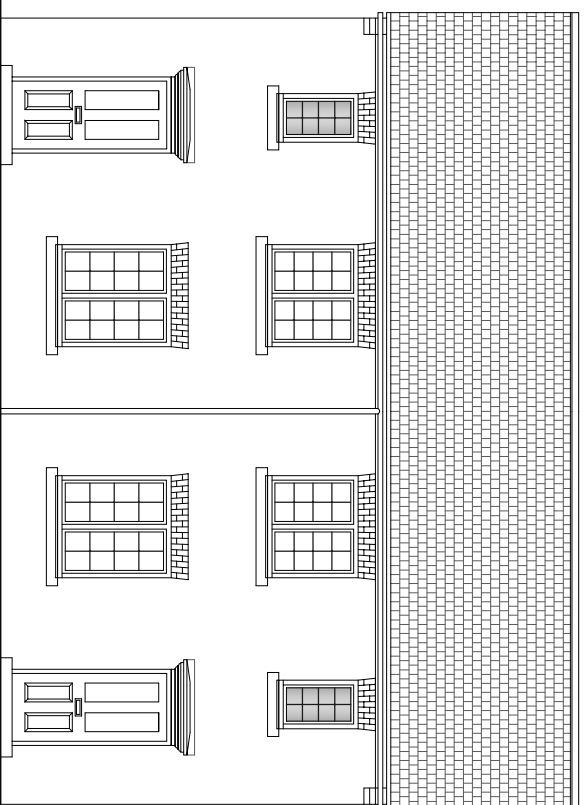
Front Elevation
