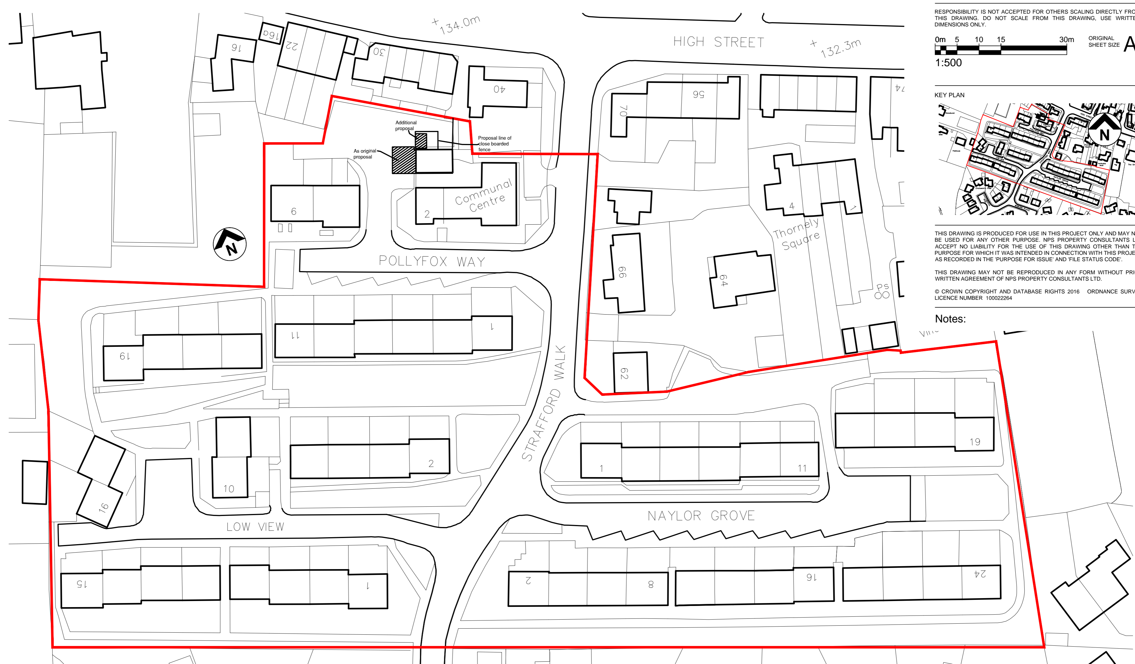
01 Site Location Plan Scale 1:500
