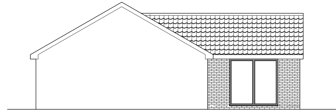
SIDE ELEVATION
