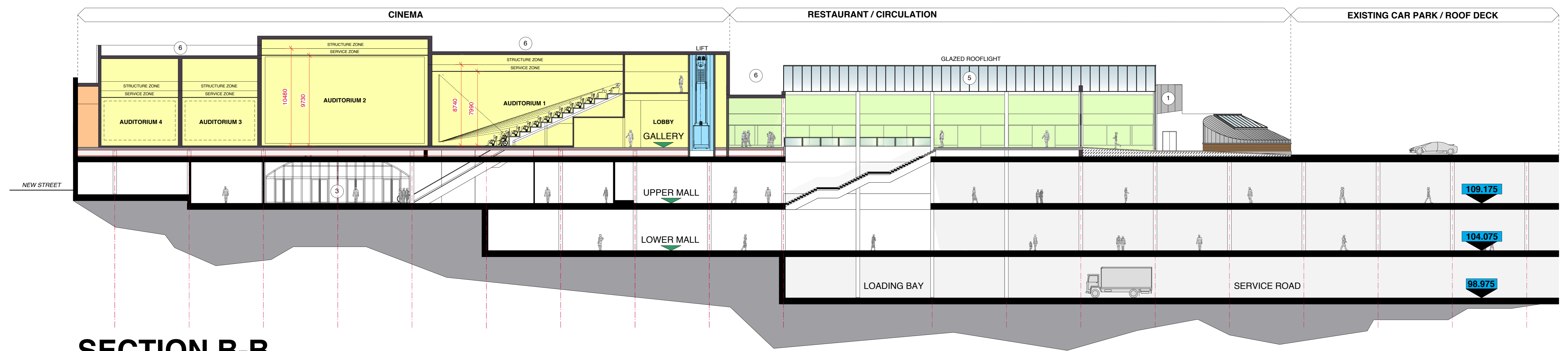
SECTION B-B
