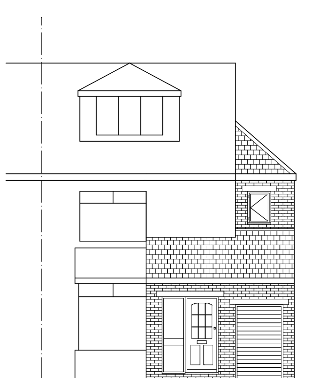
FRONT ELEVATION
