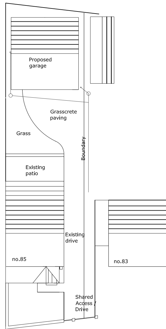
PROPOSED SITE LAYOUT
