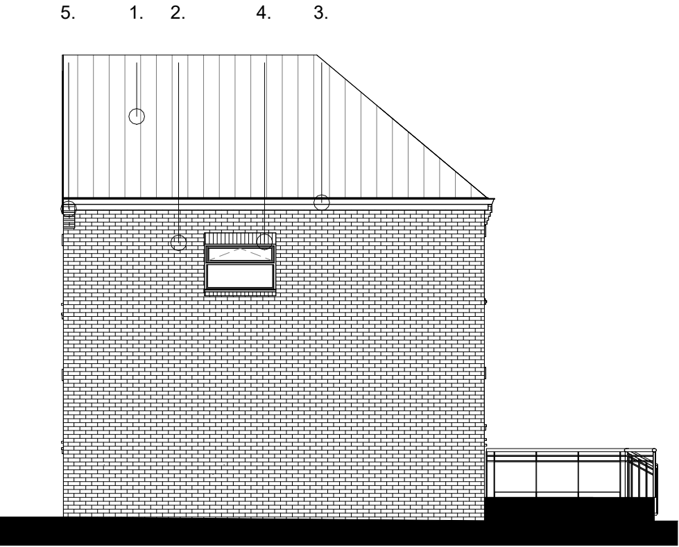
East Elevation 1 : 100
