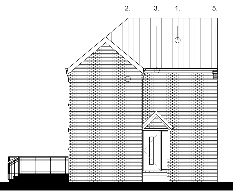
West Elevation 1 : 100
