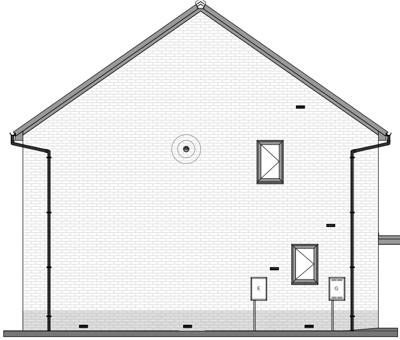
LEFT ELEVATION
